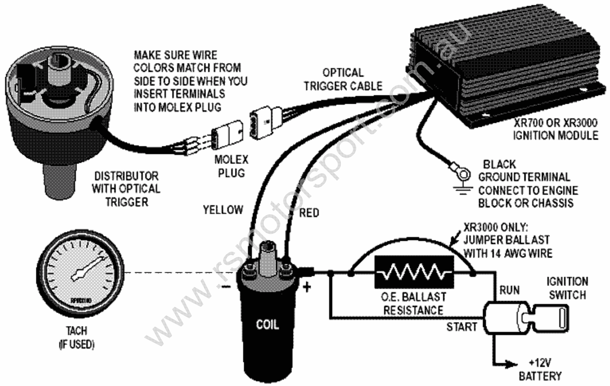
Figure 19. Basic XR700 and XR3000 Hookup
